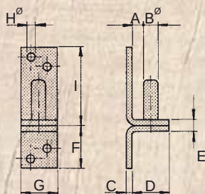
Ref. 134 (SIN MANO) / (WITHOUT HANDLE)
