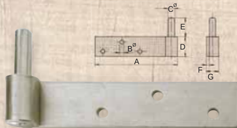
Ref. 147 (CON MANO) / (WITH HANDLE)
